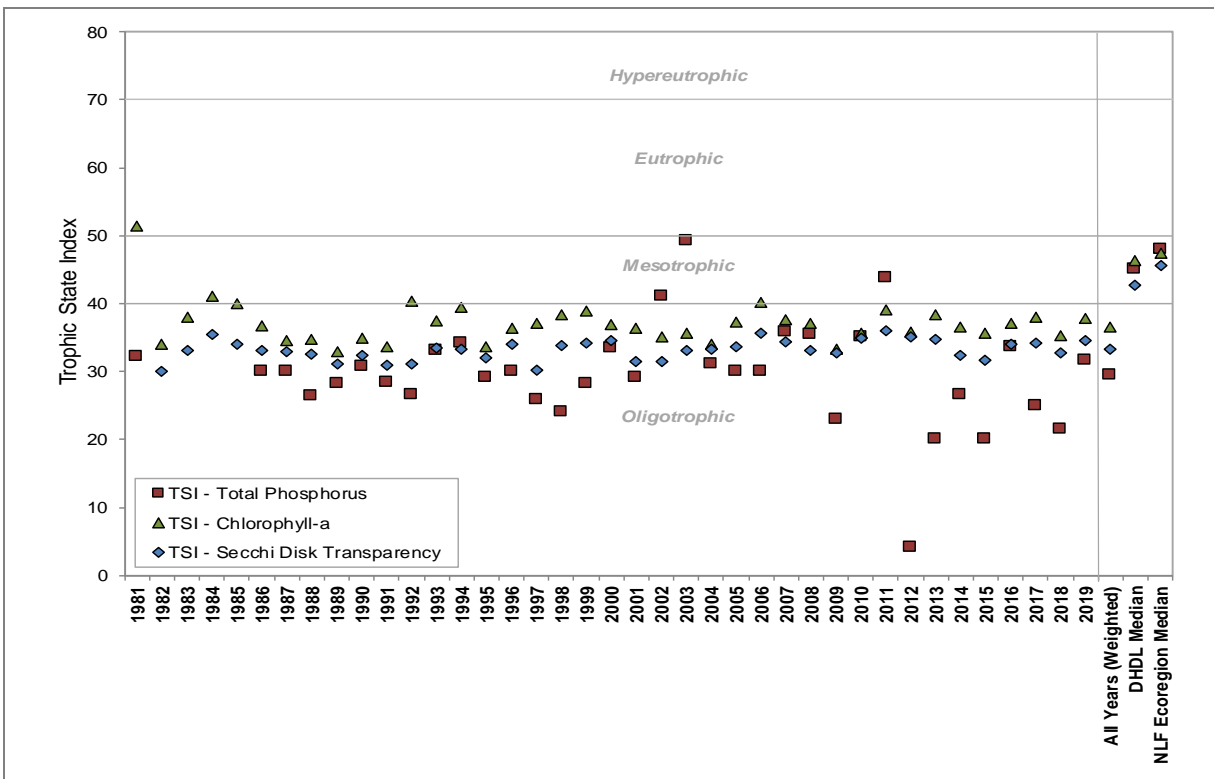
Figure 8.9.1-4. Big Muskellunge Lake, statewide deep headwater drainage lakes, and regional Trophic State Index values. Values calculated with summer month surface sample data using WDNR PUB-WT-193.
