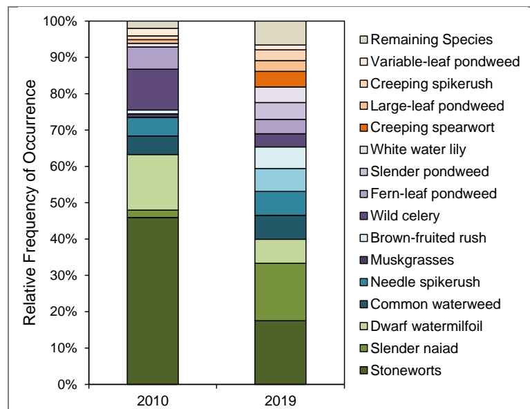
Figure 8.9.4-5. Relative frequency of occurrence of aquatic vegetation in Big Muskellunge Lake. Created using data from 2010 and 2019 point-intercept surveys.
