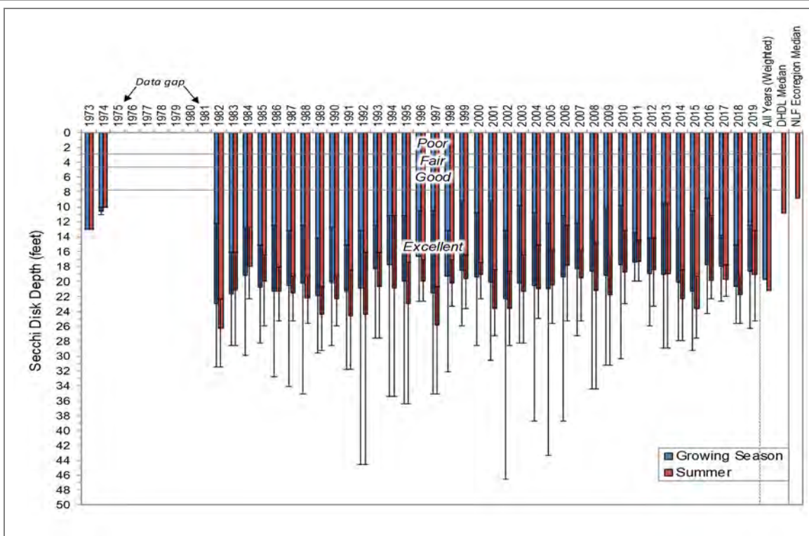
Figure 8.9.1-3. Big Muskellunge Lake, statewide deep headwater drainage lakes, and regional Secchi disk clarity values. Mean values calculated with summer month surface sample data. Water Quality Index values adapted from WDNR PUB WT-913.
