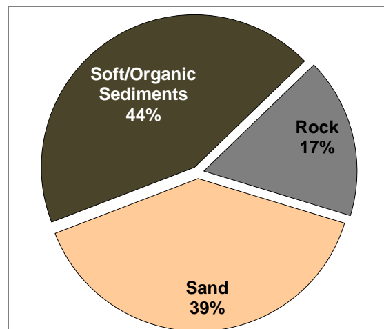
Figure 8.9.4-1. Big Muskellunge Lake 2019 proportion of substrate types in water less than 15 feet deep.
