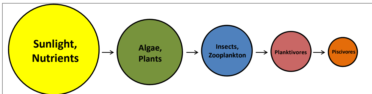
Figure 8.9.6-1. Aquatic food chain. Adapted from Carpenter et. al 1985.
